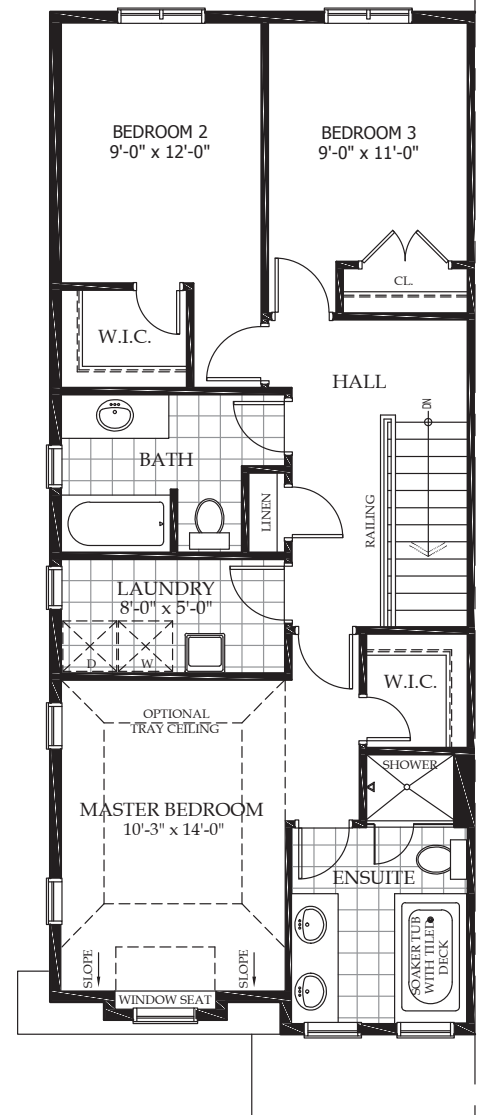
3 BEDROOM - OPT. B UPPER LEVEL 915 SQ.FT.
