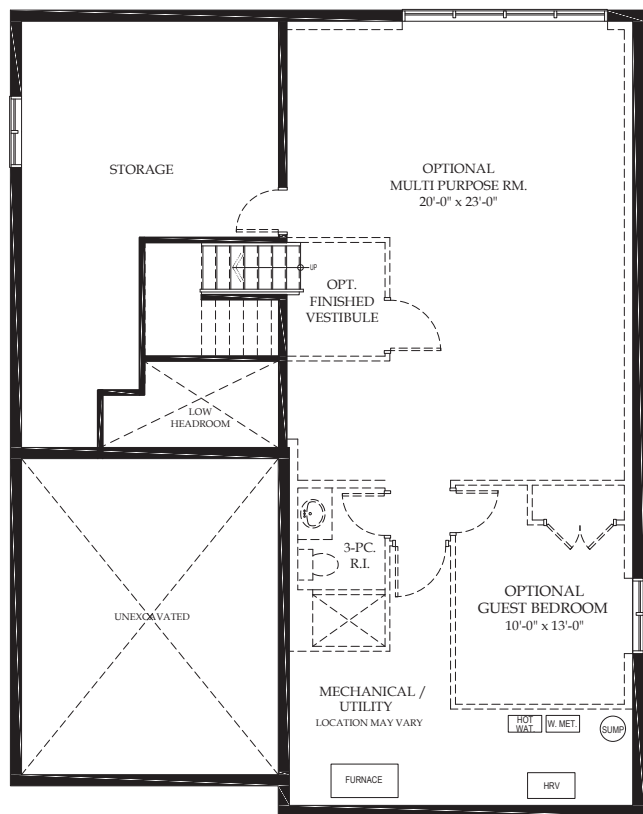
LOWER LEVEL OPTIONAL FINISHED AREA OF 700 SQ.FT. OPTIONAL FINISHED VESTIBULE AREA OF 37 SQ.FT.
