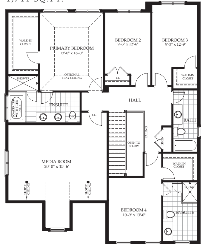
4 BEDROOM + MEDIA ROOM UPPER LEVEL 1,744 SQ.FT.
