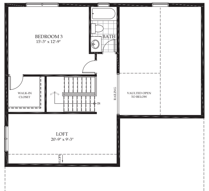
+1 BEDROOM LOFT OPT. B 677 SQ. FT.
