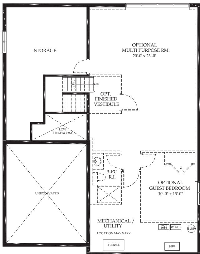
LOWER LEVEL OPTIONAL FINISHED AREA OF 700 SQ. FT.
